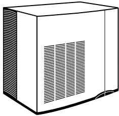
W 30" D 24.50" H 26.50" RN-1000: *1083 lbs. daily at 70/50° *821 lbs. daily at 90/70° RN-1400: *1278 lbs. daily at 70/50° *979 lbs. daily at 90/70°
