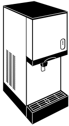
W 16.25" D 24" H 35" *300 lbs. daily at 70/50° *236 lbs. daily at 90/70°
