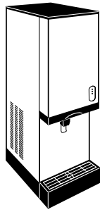
W 16.25" D 24" H 42" *300 lbs. daily at 70/50° *236 lbs. daily at 90/70°
